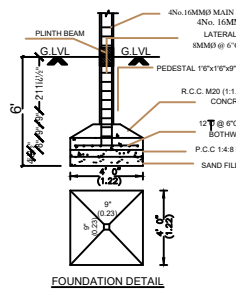
FOUNDATION DETAIL
