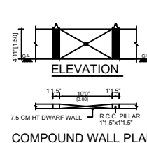
COMPOUND WALL PLAN
