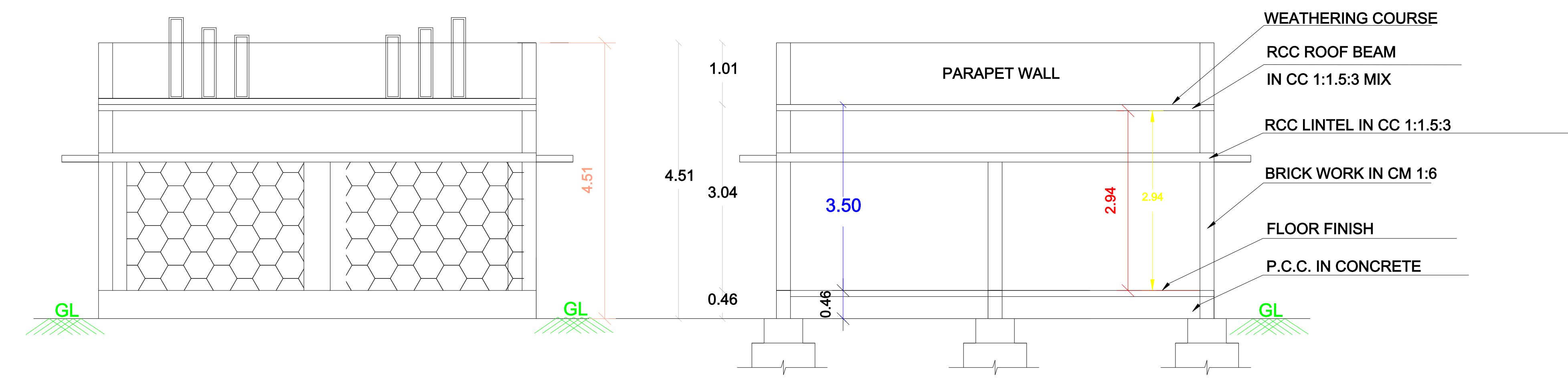
FRONT ELEVATION
