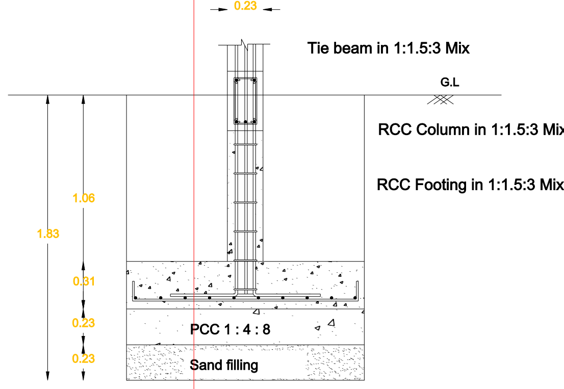
FOUNDATION DETAILS
