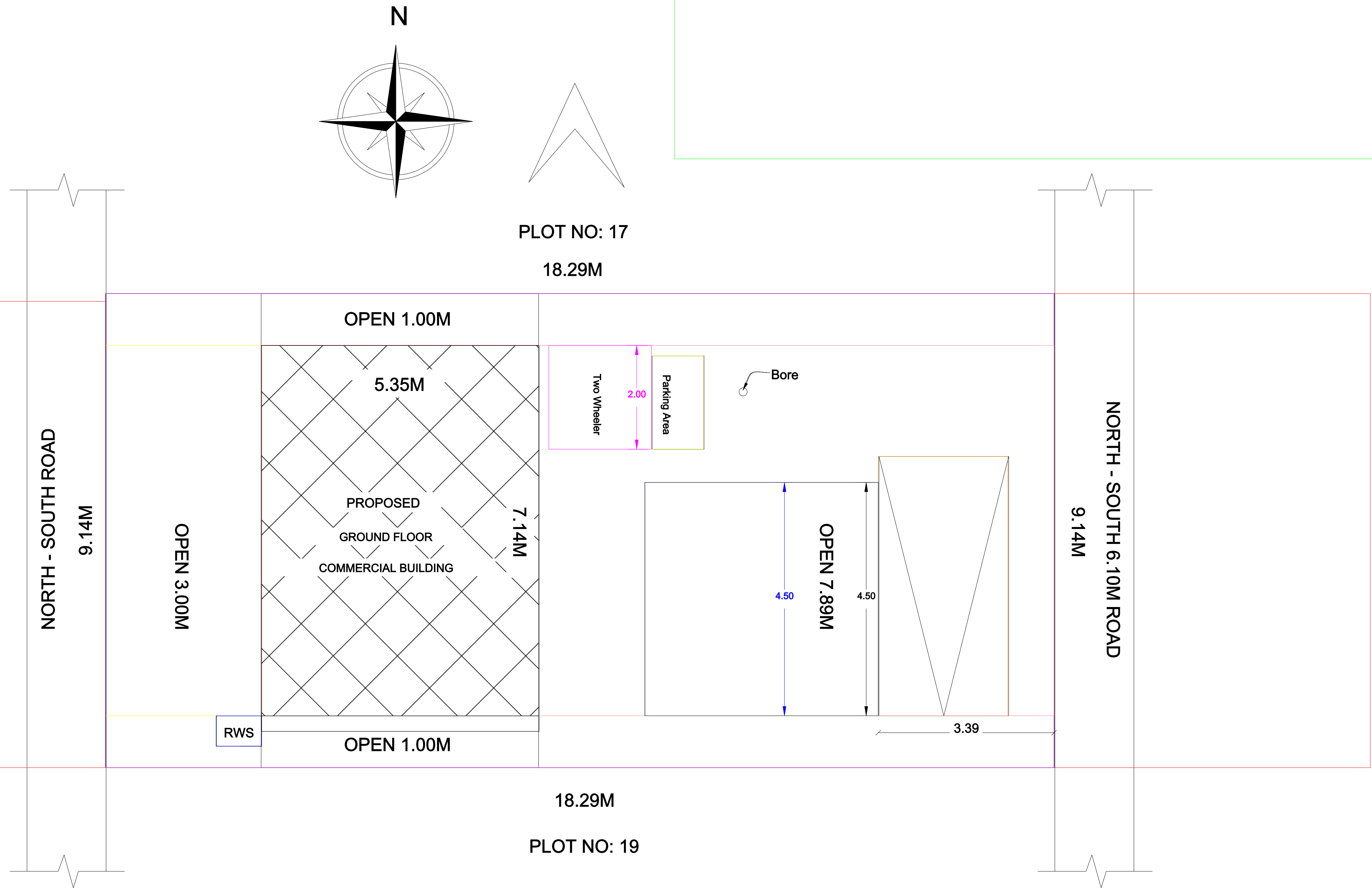
SITE PLAN
