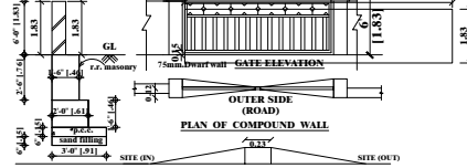
COMPOUND WALL & GATE DETAIL
