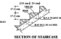
SECTION OF STAIRCASE
