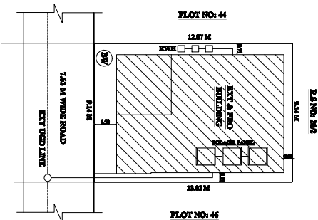
SITE P/LA SCALE:- 1:100
