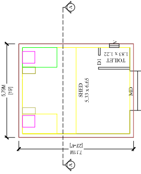
PRO.GROUND FLOOR PLAN
