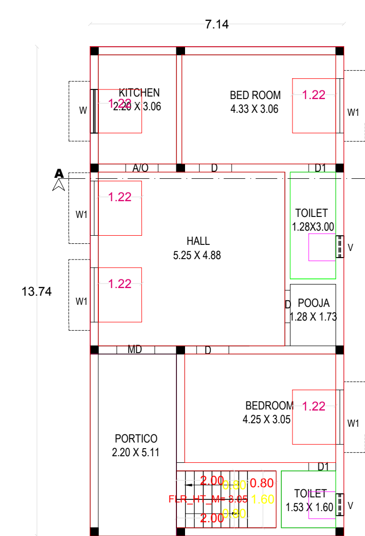
GROUND FLOOR PLAN (North Facing)
