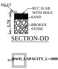
PLAN OF RWH
