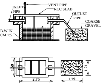
SEPTIC TANK & D-TRENCH DETAILS (NOT TO SCALE)
