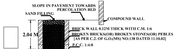
SECTION OF RAIN WATER PERCOLATION BED
