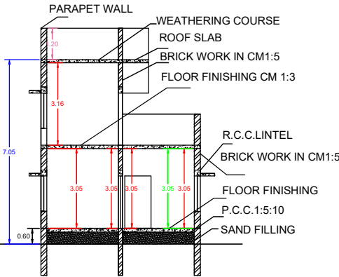
SECTION ON SS
