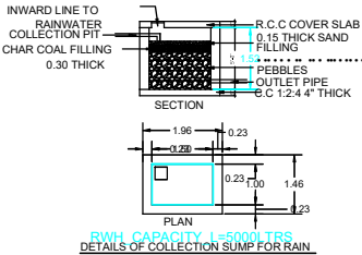
DETAILS OF COLLECTION SUMP FOR RAIN
