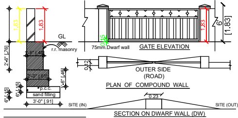
SECTION ON DWARF WALL (DW)
