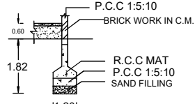
FOUNDATION DETAILS
