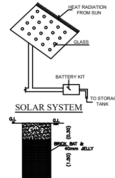
SOLAR SYSTEM RAIN WATER HARVESTING SYSTEM
