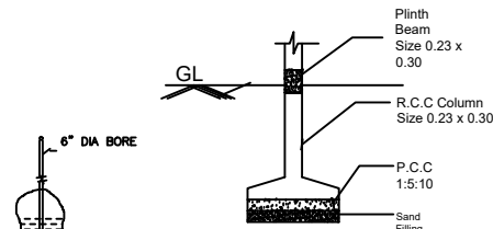
FOUNDATION DETAILS
