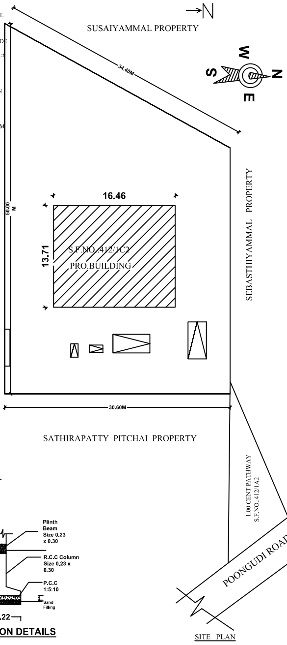
SITE PLAN
