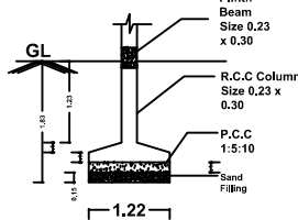
FOUNDATION DETAILS
