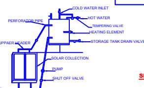
DETAILS OF SOLAR WATER HARVESTING (NTS)
