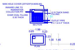
DETAILS OF RAINWATER HARVESTING
