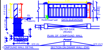
DETAILS OF COMPOUND WALL
