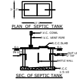
SEC. OF SEPTIC TANK
