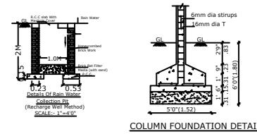
COLUMN FOUNDATION DETAIL
