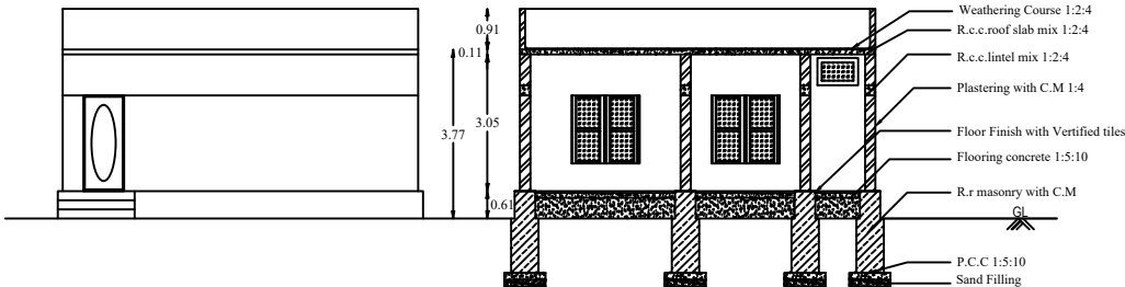
ELEVATION (NORTH SIDE)
