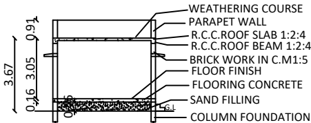
SECTION- SS
