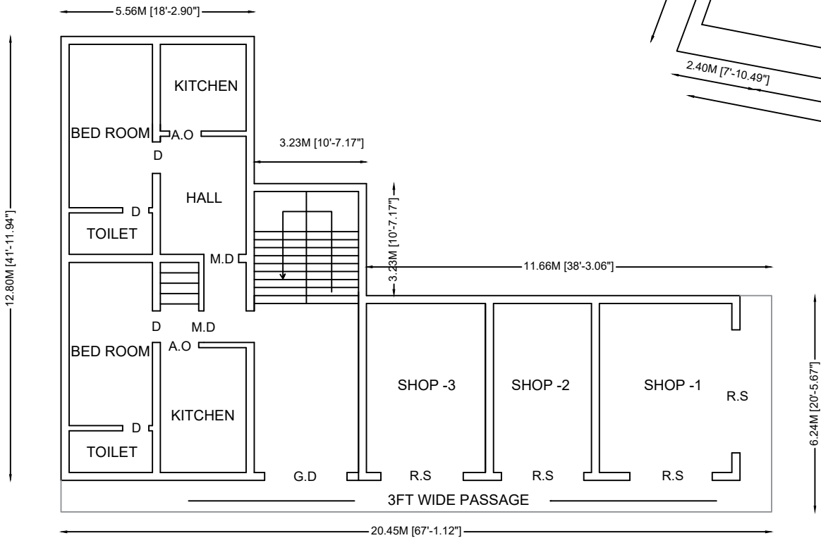
PROPOSED FRIST FLOOR PLAN
