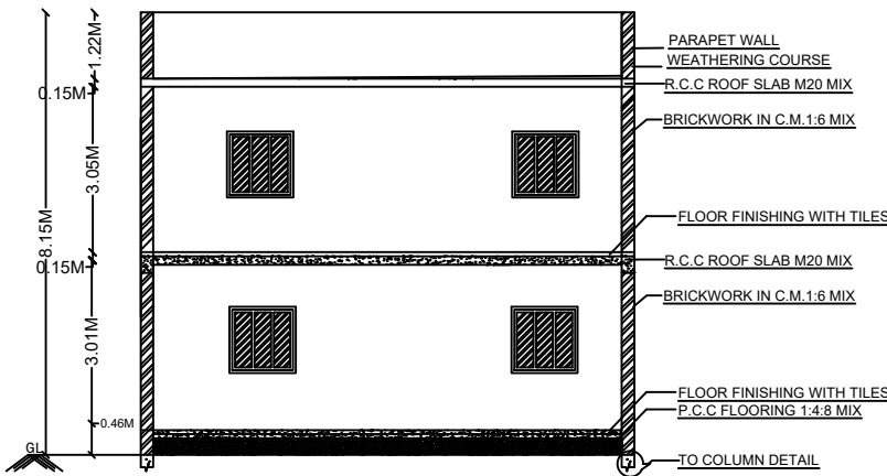
SECTION A - B
