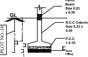
FOUNDATION DETAILS
