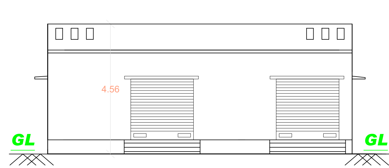
FRONT ELEVATION
