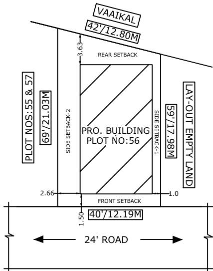
SITE PLAN
