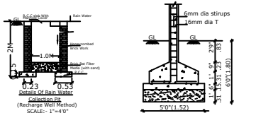
COLUMN FOUNDATION DETAIL
