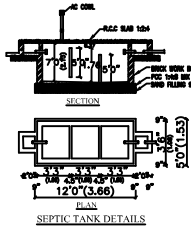
SEPTIC TANK DETAILS
