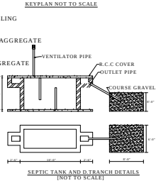
SEPTIC TANK AND DRAIN DETAILS [NOT TO SCALE]
