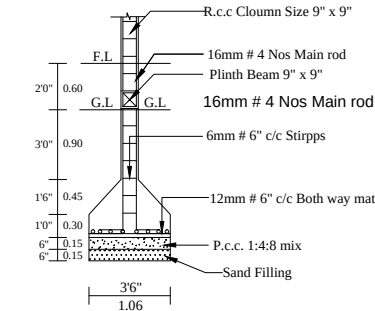
COLUMN DETIAL
