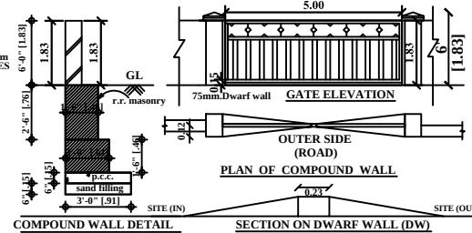
COMPOUND WALL DETAIL PLAN OF COMPOUND WALL SECTION ON DWARF WALL (DW)
