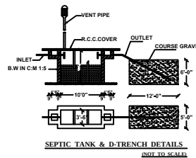
SEPTIC TANK & D-TRENCH DETAILS (NOT TO SCALE)
