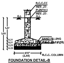
FOUNDATION DETAIL-B
