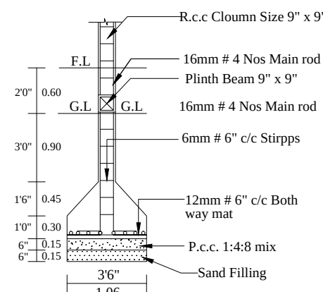
COLUMN DETAILS
