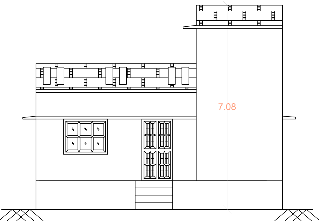
FRONT ELEVATION
