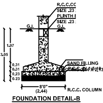
FOUNDATION DETAIL-B
