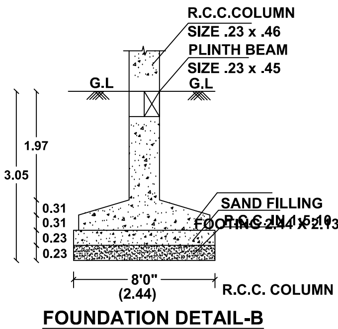
FOUNDATION DETAIL-B
