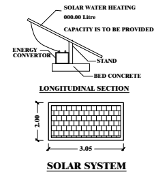
SOLAR SYSTEM
