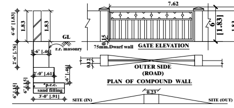
COMPOUND WALL & GATE DETAIL
