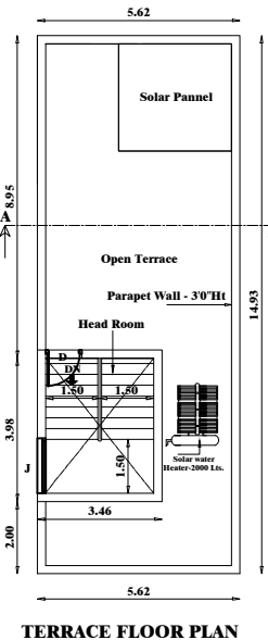
TERRACE FLOOR PLAN
