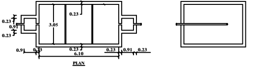
PLAN & SECTION OF SEPTIC TANK & DISPERSION TRENCH
