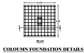
COLOUMN FOUNDATION DETAILS
