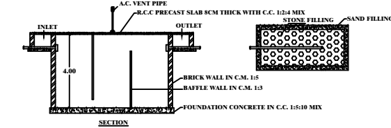
SECTION OF RAIN WATER PERCOLATION BED RWV_CAPACITY_L=5000LTRS
