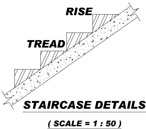
STAIRCASE DETAILS (SCALE = 1 : 50 )
