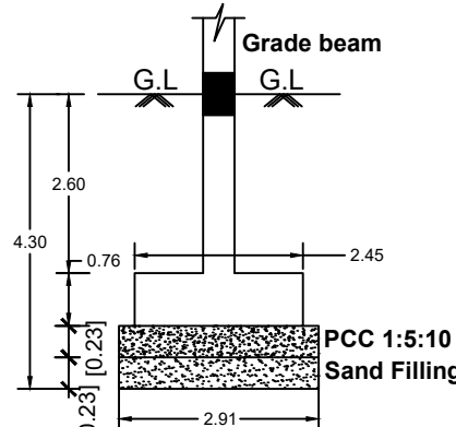
FOUNDATION DETAILS
