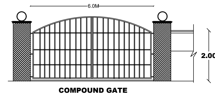
COMPOUND GATE
