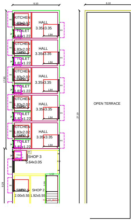
PROPOSED 1 ST FLOOR PLAN
