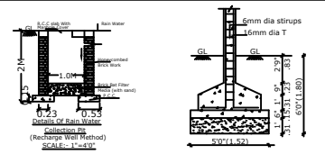
COLUMN FOUNDATION DETAIL
