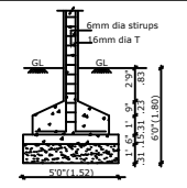
COLUMN FOUNDATION DETAIL
