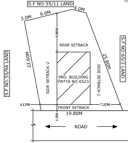
SITE PLAN
