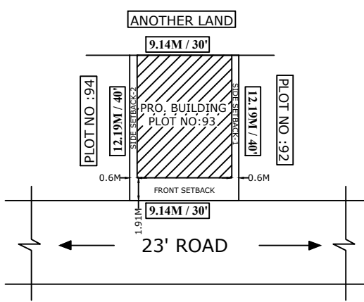
SITE PLAN
