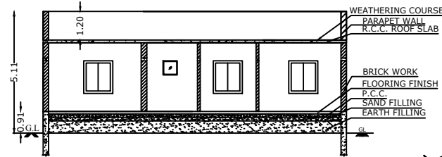
SECTION ON XX
