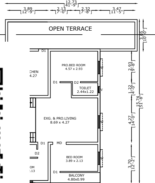
RO. FIRST FLOOR PLAN
