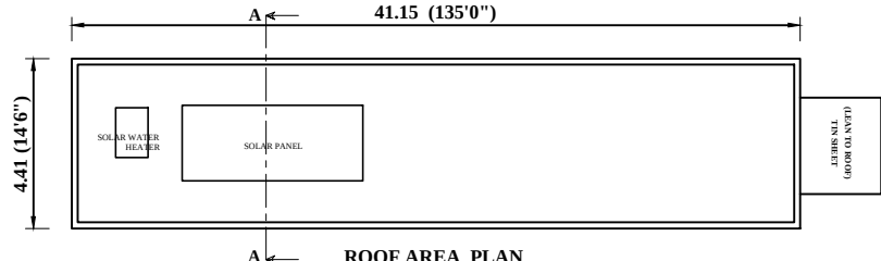
ROOF AREA PLAN
