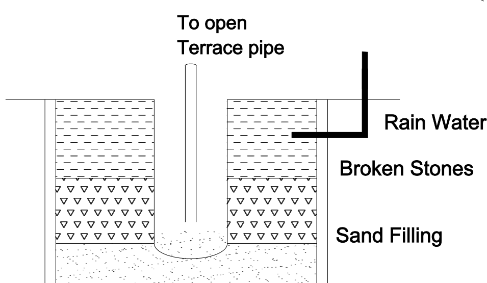
RAIN WATER COLLECTION CHAMBER
