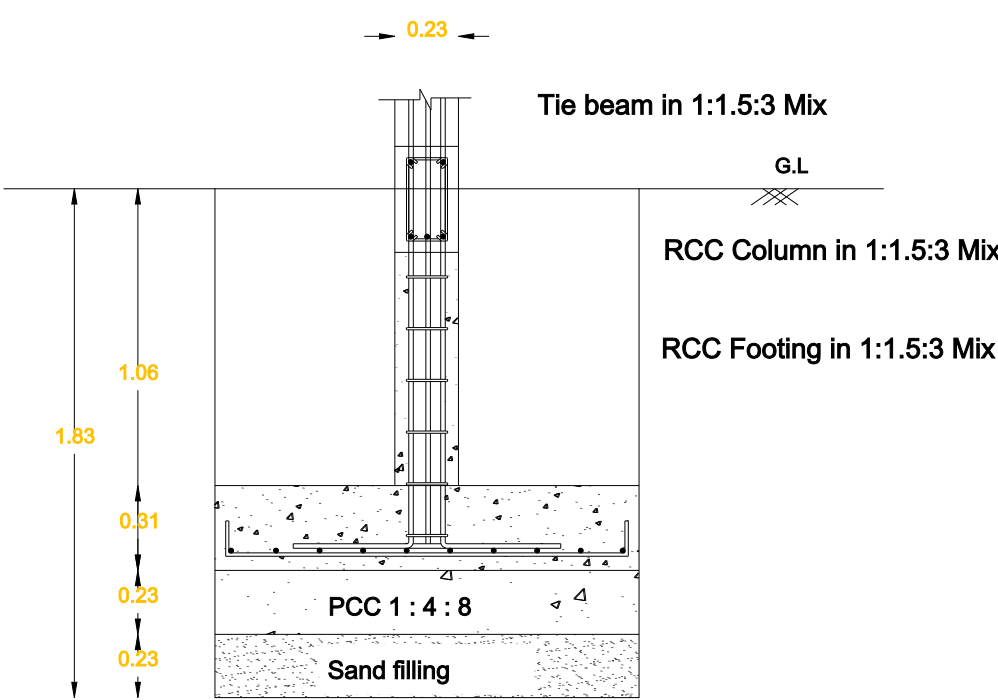
FOUNDATION DETAILS
