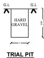
TRIAL PIT
