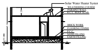
SECTION ON XX
