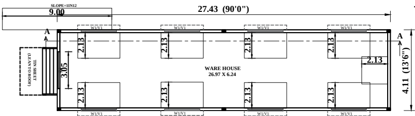
PROPOSED BUILDING PLAN
