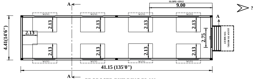
PROPOSED BUILDING PLAN
