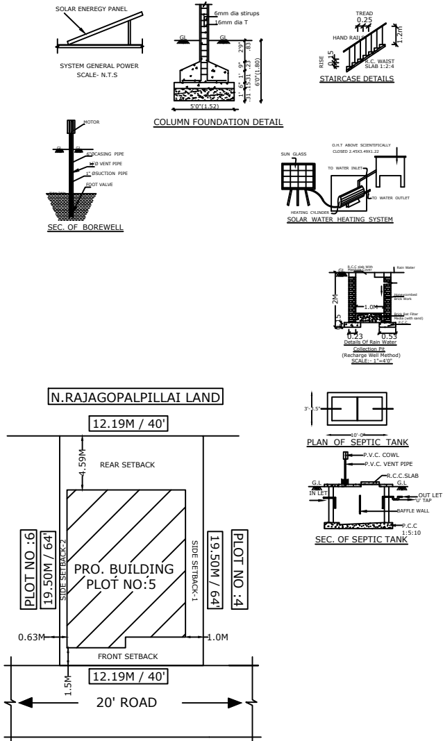
SITE PLAN
