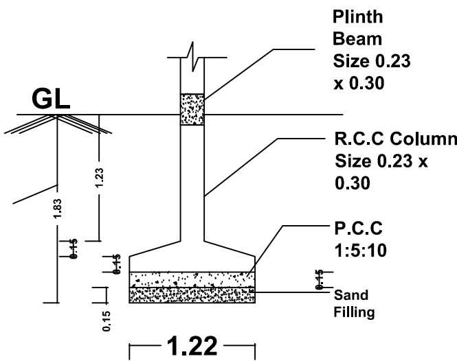
FOUNDATION DETAILS
