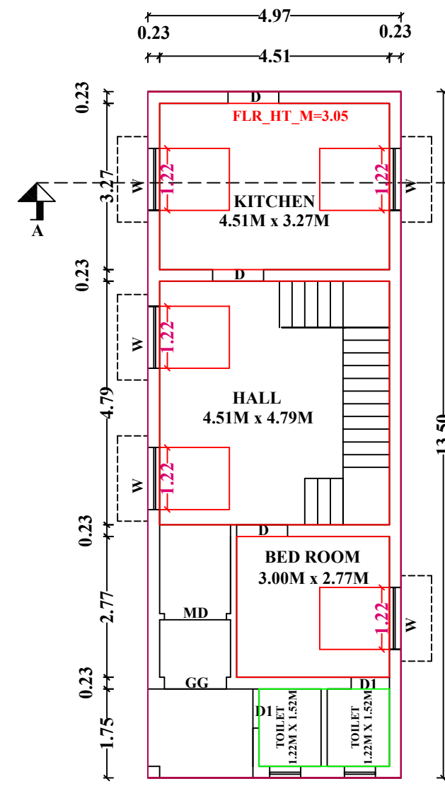
FLOOR-GROUND PRO.GROUND FLOOR PLAN
