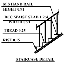
STAIRCASE DETAIL
