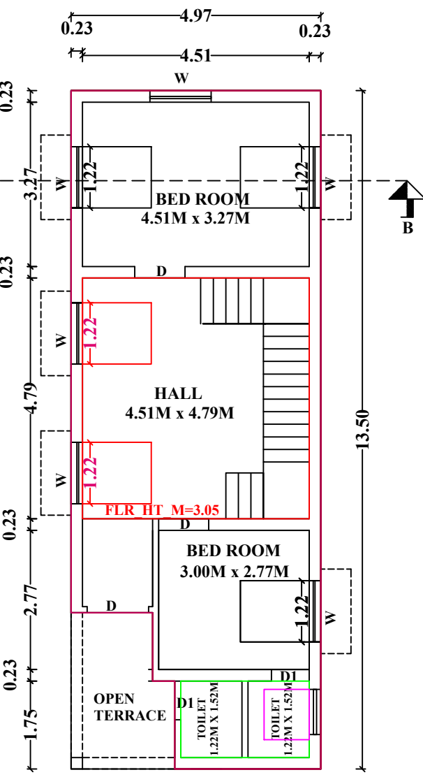
FLOOR-1 PRO.FIRST FLOOR PLAN
