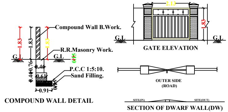
SECTION OF DWARF WALL(DW)
