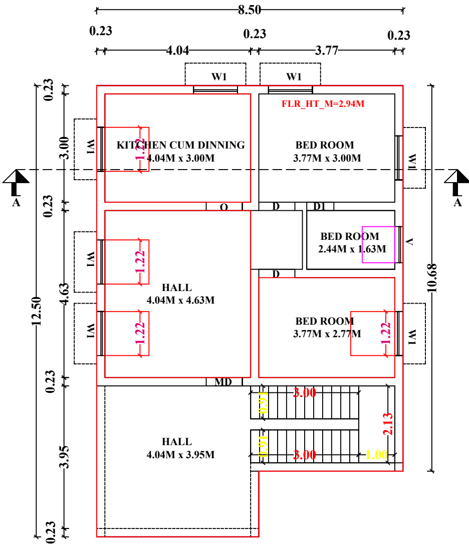
FLOOR-0
