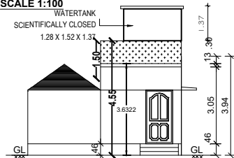
PROPOSED ELEVATION
