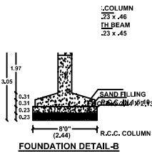
FOUNDATION DETAIL-B
