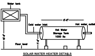
SOLAR WATER HEATER DETAILS
