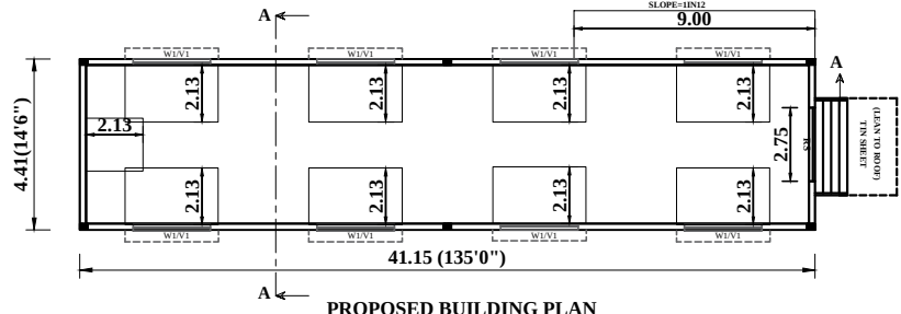
PROPOSED BUILDING PLAN
