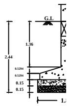
COLUMN FOUNDATION (DETAILED)
