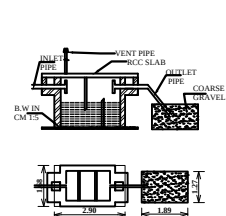
SEPTIC TANK & D-TRENCH DETAILS (NOT TO SCALE)
