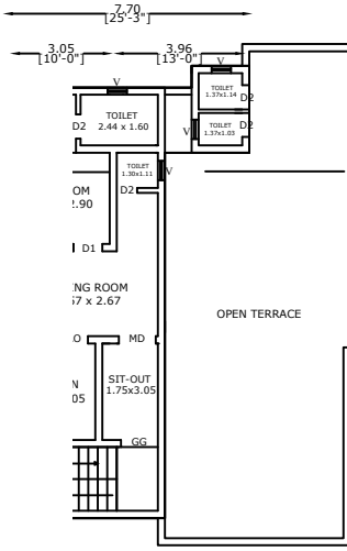
& PRO. FIRST FLOOR PLAN
