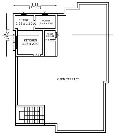
PRO. SECOND FLOOR PLAN
