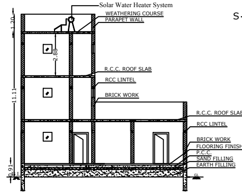
SECTION ON XX
